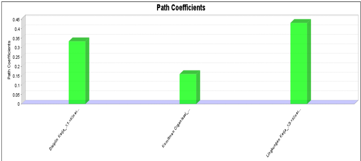
Gambar 3. Hasil Path Coefficients
