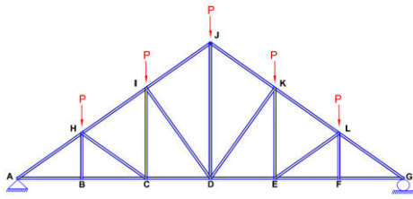
Gambar 3.5 Tipe Howe
