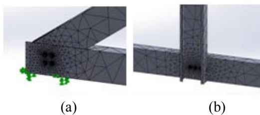
Gambar 4.1 Meshing Tipe Howe
