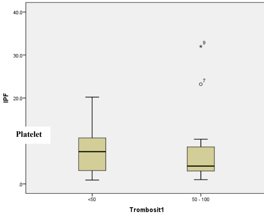
Figure 2. IPF level in mild and moderate-severe thrombocytopenia groups
