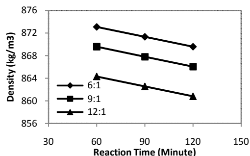
Fig. 3. Effect of Reaction Time on Density at Reaction Temperature of 55°C and Amount of Catalysts of 3%
