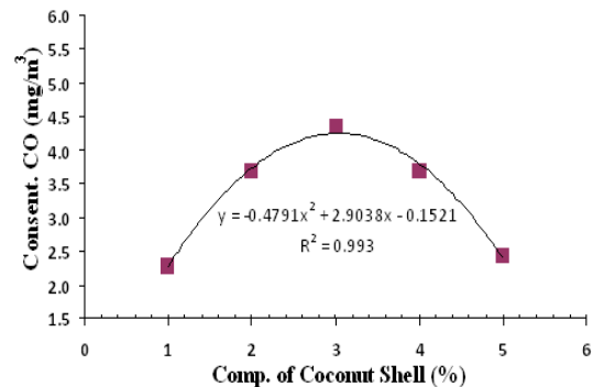
Figure 3. Influence of Composition Ratio Straw Rice And Coconut Shell To CO Emissions
